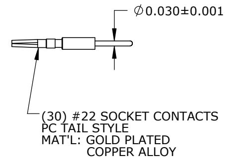
PANEL CONNECTOR, FEMALE MAT'L: UV PBT, BLACK
