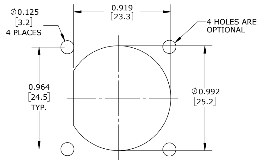
RECOMMENDED PANEL CUT-OUT TOLERANCE: \pm 0.003 [0.008]
