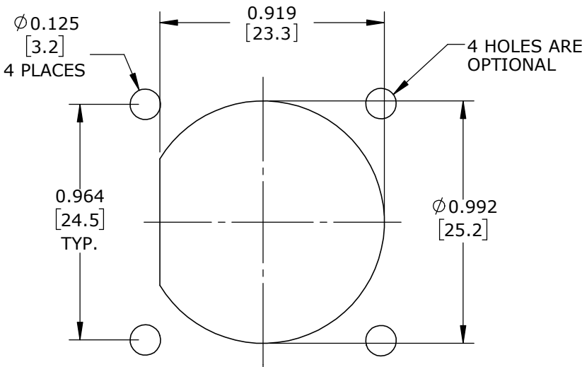
RECOMMENDED PANEL CUT-OUT TOLERANCE: ±.003 [0.008]
