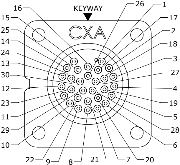
WIRE VIEW
