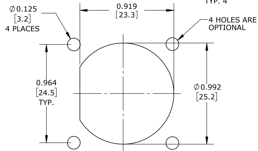
RECOMMENDED PANEL CUT-OUT TOLERANCE: \pm 0.003 [0.008]
