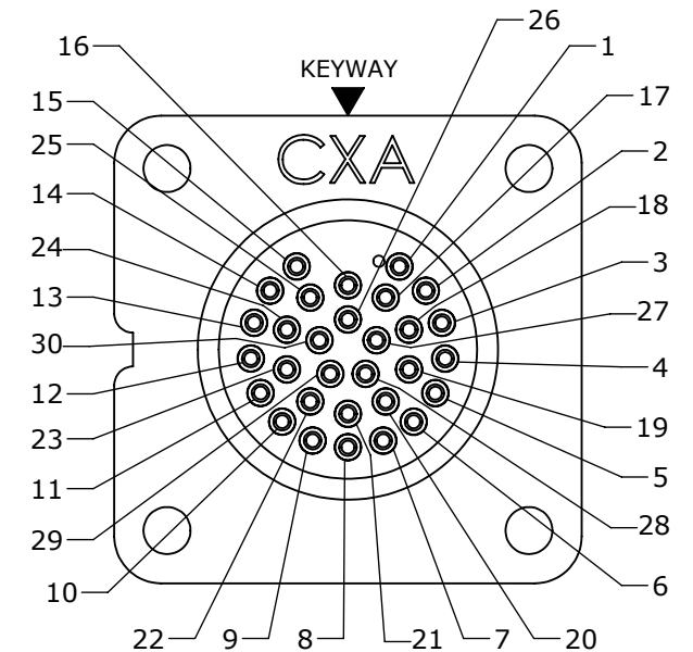
WIRE VIEW
