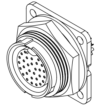
ASSEMBLED VIEW
