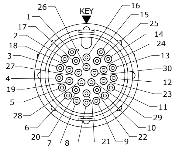
FACE VIEW
