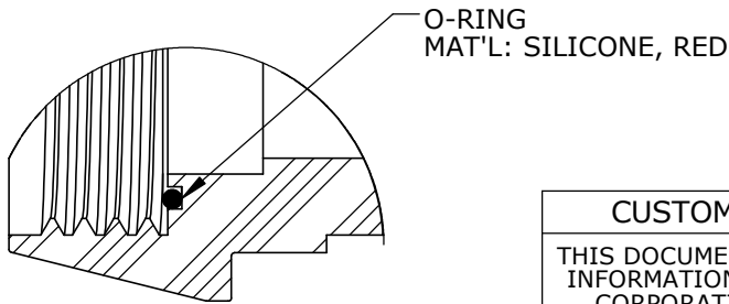
DETAIL A
