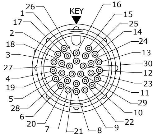
FACE VIEW
