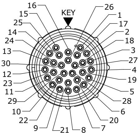
WIRE VIEW
