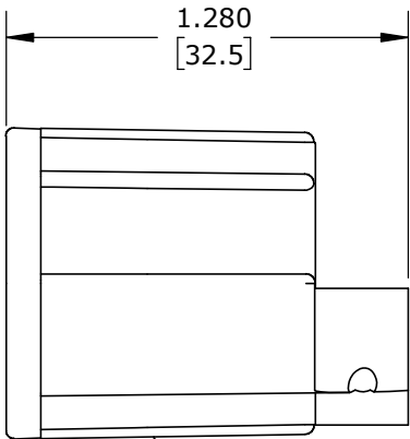
BACKSHELL MAT'L: UV PBT, BLACK
