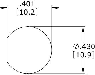
RECOMMENDED PANEL CUT-OUT TOLERANCE: ±.003
