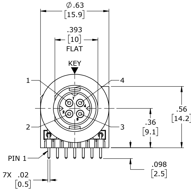
FACE VIEW
