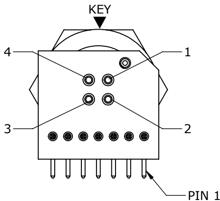
WIRE VIEW
