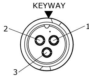
FACE VIEW W3180-3SG-P-4XX
