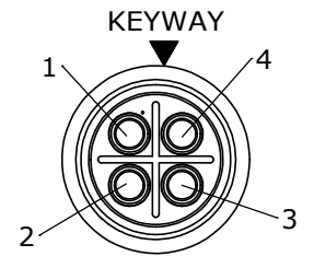
WIRE VIEW W3180-4SG-P-4XX
