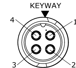
FACE VIEW W3180-4SG-P-4XX
