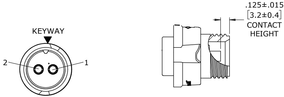
FACE VIEW W3180-2SG-P-4XX
