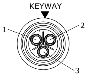
WIRE VIEW W3180-3SG-P-4XX
