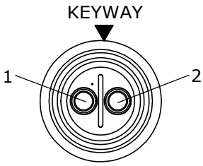
WIRE VIEW W3180-2SG-P-4XX
