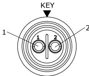
WIRE VIEW
