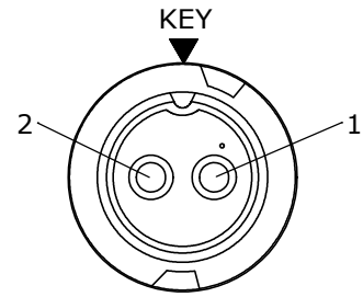
FACE VIEW
