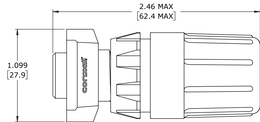
SHOWN ASSEMBLED FOR CUSTOMER REFERENCE ONLY
