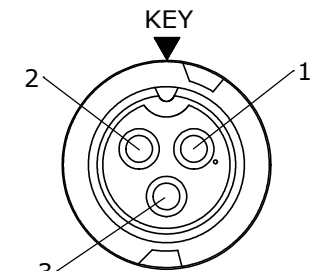
FACE VIEW
