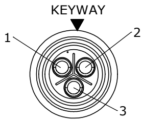
WIRE VIEW W3182-3SG-P-4XX
