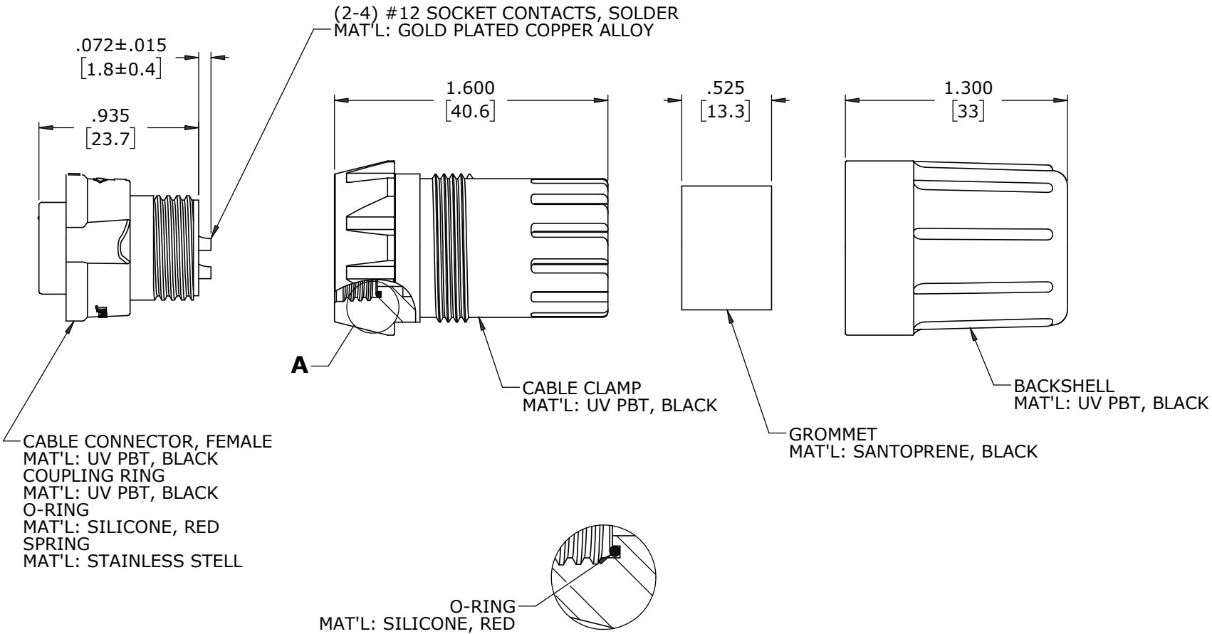
DETAIL A
