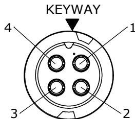
FACE VIEW W3182-4SG-P-4XX
