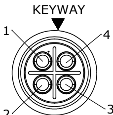
WIRE VIEW W3182-4SG-P-4XX
