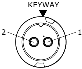
FACE VIEW W3182-2SG-P-4XX
