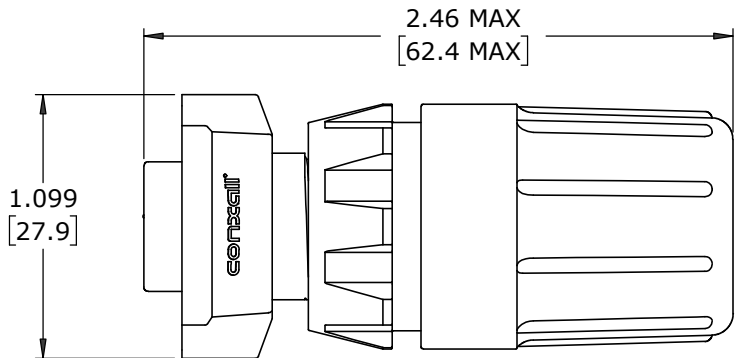
SHOWN ASSEMBLED FOR CUSTOMER REFERENCE ONLY
