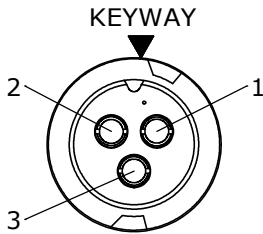
FACE VIEW W3182-3SG-P-4XX
