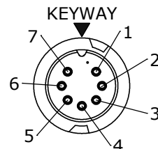
FACE VIEW W3280-7SG-P-4XX
