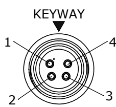
WIRE VIEW W3280-4SG-P-4XX
