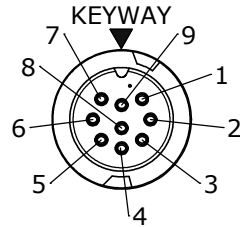
FACE VIEW W3280-9SG-P-4XX
