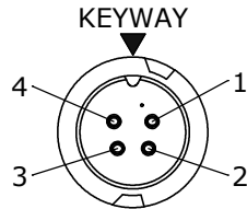
FACE VIEW W3280-4SG-P-4XX
