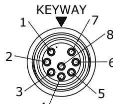
WIRE VIEW W3280-8SG-P-4XX
