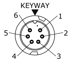
FACE VIEW W3280-6SG-P-4XX
