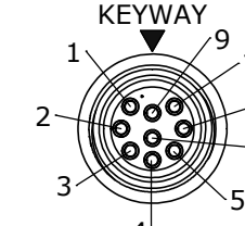
WIRE VIEW W3280-9SG-P-4XX
