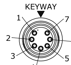
WIRE VIEW W3280-7SG-P-4XX
