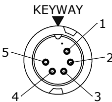
FACE VIEW W3280-5SG-P-4XX
