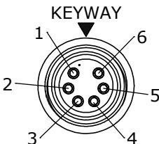
WIRE VIEW W3280-6SG-P-4XX
