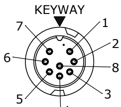
FACE VIEW W3280-8SG-P-4XX
