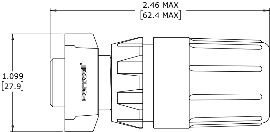
SHOWN ASSEMBLED FOR CUSTOMER REFERENCE ONLY
