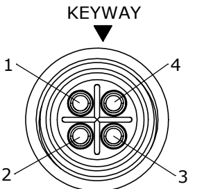
WIRE VIEW W3382-4SG-P-4XX
