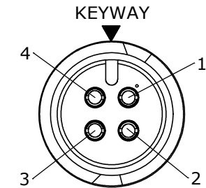
FACE VIEW W3382-4SG-P-4XX
