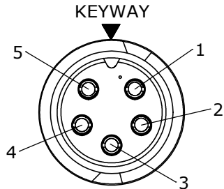
FACE VIEW W3382-5SG-P-4XX
