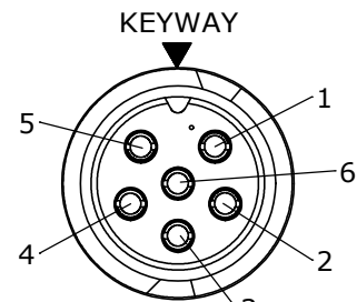
FACE VIEW W3382-6SG-P-4XX
