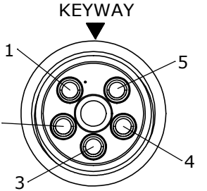
WIRE VIEW W3382-5SG-P-4XX
