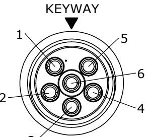
WIRE VIEW W3382-6SG-P-4XX
