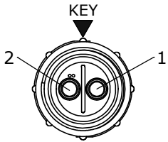
WIRE VIEW W5180-3SG-P-4XX
