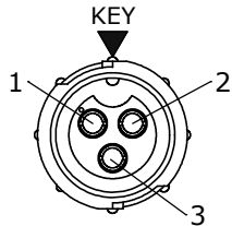
FACE VIEW W5180-3SG-P-4XX
