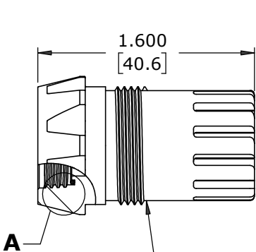
CABLE CLAMP MAT'L: UV PBT, BLACK
