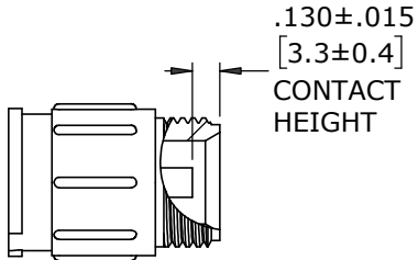
(2-3) #12 SOCKET CONTACTS, CRIMP MAT'L: COPPER ALLOY, GOLD PLATED
