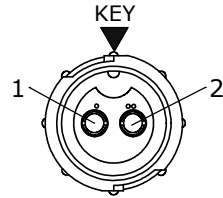
FACE VIEW W5182-2SG-P-4XX
