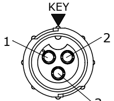
FACE VIEW W5182-3SG-P-4XX
