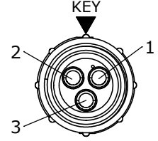
WIRE VIEW W5182-3SG-P-4XX
