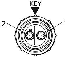
WIRE VIEW W5182-2SG-P-4XX
