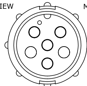
W5380-6PG-P-5XX MATING VIEW
