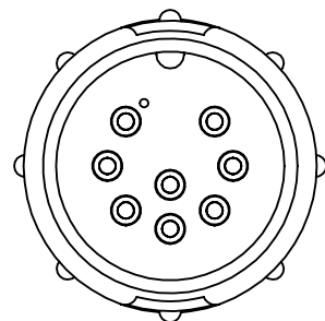
W5280-8PG-P-5XX MATING VIEW
