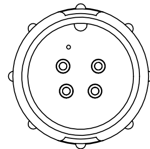
W5280-4PG-P-5XX MATING VIEW
