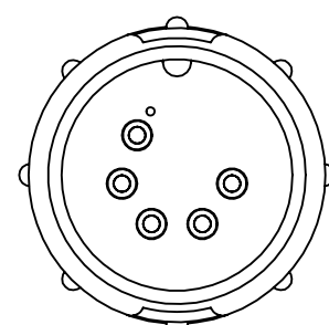
W5280-5PG-P-5XX MATING VIEW
