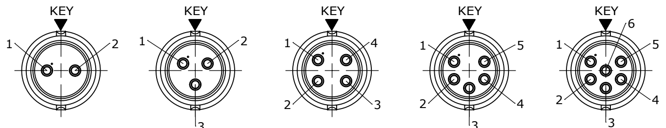
WIRING END W6280-2PG-P-5XX WIRING END W6280-3PG-P-5XX WIRING END W6280-4PG-P-5XX WIRING END W6280-5PG-P-5XX WIRING END W6280-6PG-P-5XX
