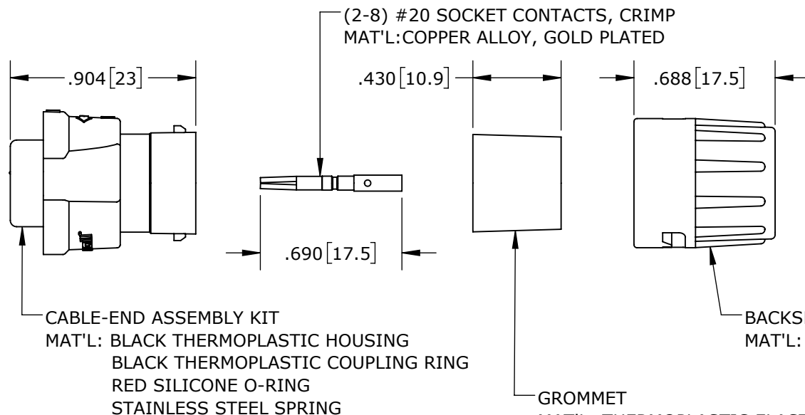
SHOWN ASSEMBLED KIT ASSY: W6280-2SG-P-3XX SHOWN
