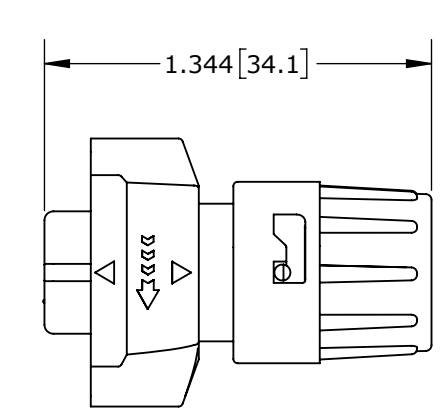
SHOWN ASSEMBLED KIT ASSY: W6280-2SG-P-3XX SHOWN
