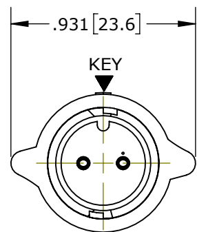
MATING FACE ASSY: W6282-2SG-P-5XX SHOWN
