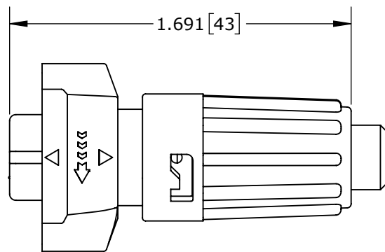
SHOWN ASSEMBLED KIT ASSY: W6282-2SG-P-5XX SHOWN
