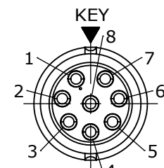
WIRING END W6282-8SG-P-5XX
