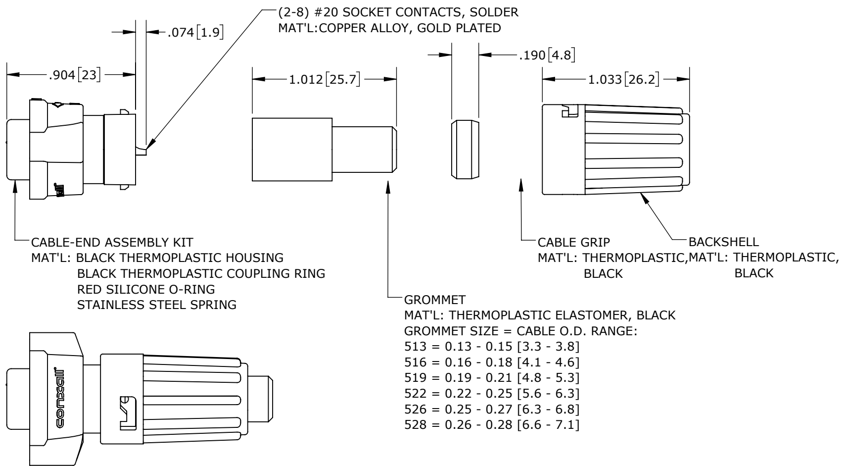
SHOWN ASSEMBLED KIT ASSY: W6282-2SG-P-5XX SHOWN
