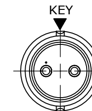
WIRING END ASSY: W6282-2SG-P-5XX SHOWN WITHOUT HARDWARE
