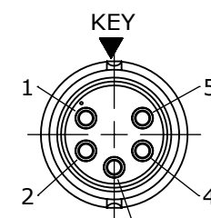
WIRING END W6280-5SG-P-5XX
