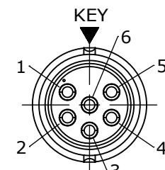
WIRING END W6282-6SG-P-5XX
