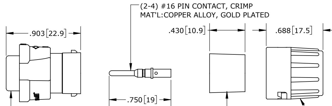
SHOWN ASSEMBLED KIT ASSY: W6380-2PG-P-3XX SHOWN
