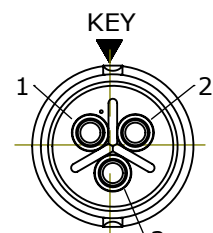
WIRING END W6380-3PG-P-3XX
