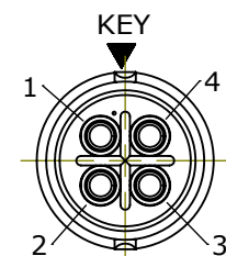
WIRING END W6380-4PG-P-3XX
