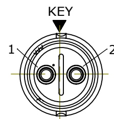
WIRING END W6380-2PG-P-3XX
