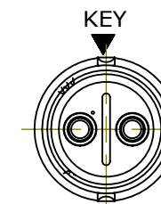
WIRING END ASSY: W6380-2PG-P-3XX SHOWN WITHOUT HARDWARE
