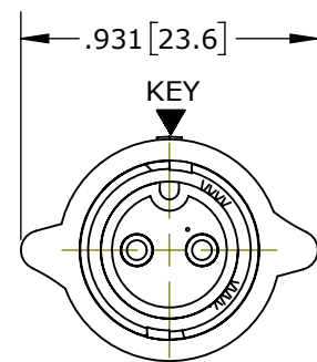
MATING FACE ASSY: W6380-2PG-P-3XX SHOWN
