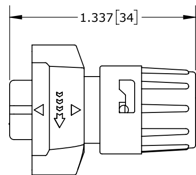
SHOWN ASSEMBLED KIT ASSY: W6380-2SG-P-3XX SHOWN
