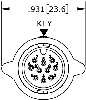
MATING FACE ASSY: W6880-10SG-P-5XX SHOWN
