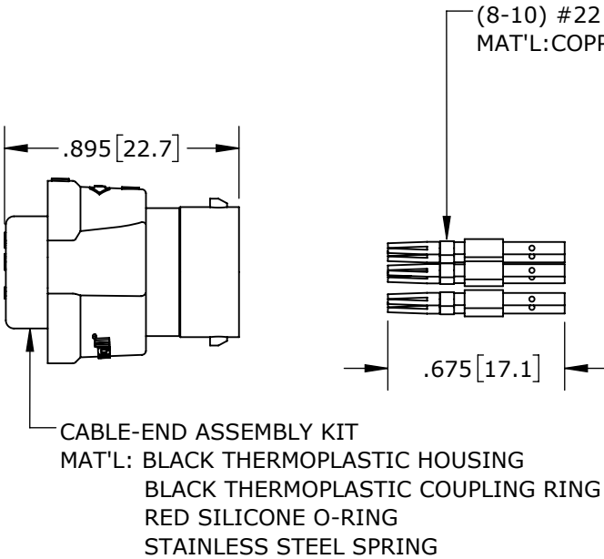
SHOWN ASSEMBLED KIT ASSY: W6880-10SG-P-5XX SHOWN
