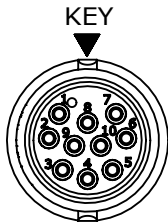
WIRING END W6880-10SG-P-5XX
