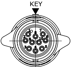
WIRING END ASSY: W6880-10SG-P-5XX SHOWN WITHOUT HARDWARE
