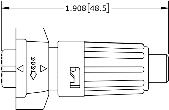
SHOWN ASSEMBLED KIT ASSY: W6880-10SG-P-5XX SHOWN
