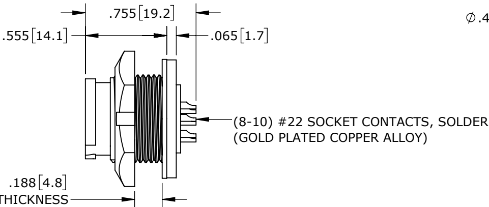
SOLDER CONTACTS W7882-10SG-P-300 SHOWN
