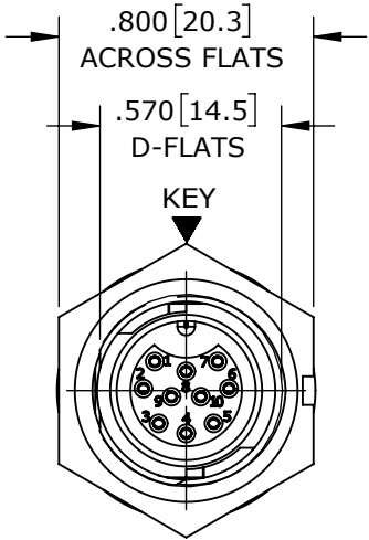
MATING FACE W7882-10SG-P-300 SHOWN
