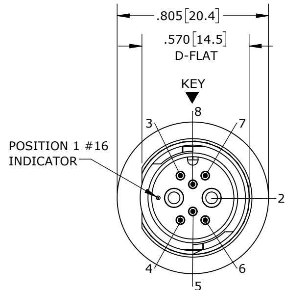
MATING FACE W7A82-8PG-P-300 SHOWN
