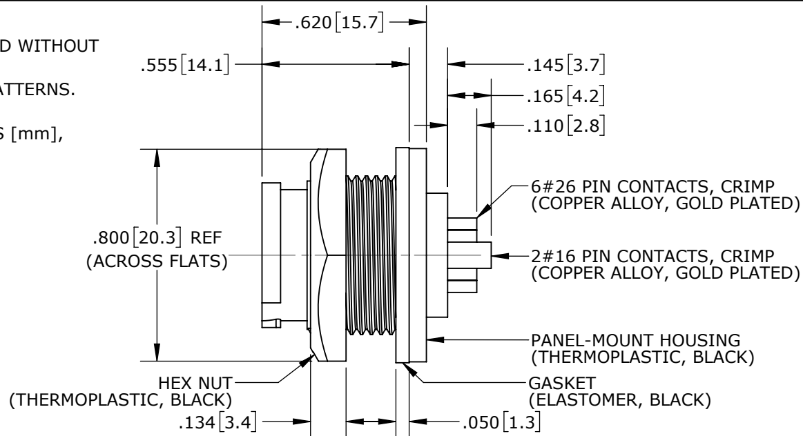
CRIMP CONTACTS (SHOWN ASSEMBLED) W7A80-8PG-P-300 SHOWN
