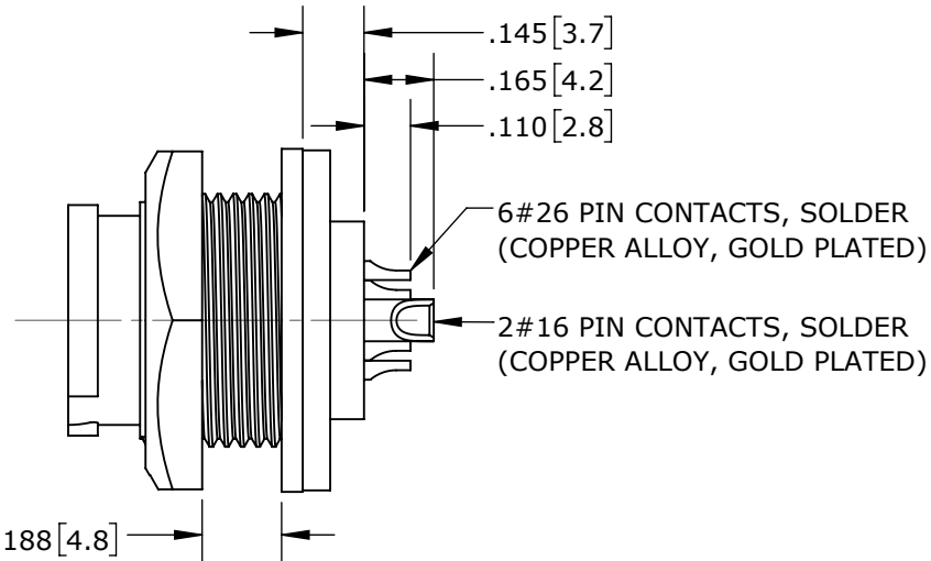
SOLDER CONTACTS W7A82-8PG-P-300 SHOWN
