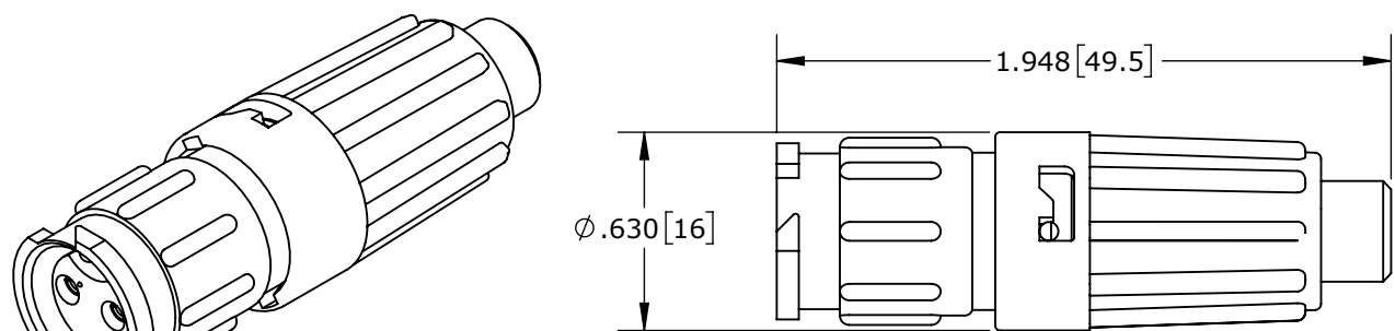
TYPICAL CABLE-TO-CABLE CONNECTOR SHOWN ASSEMBLED
