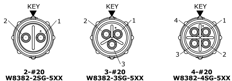
CONTACT ARRANGEMENTS (WIRING END SHOWN)
