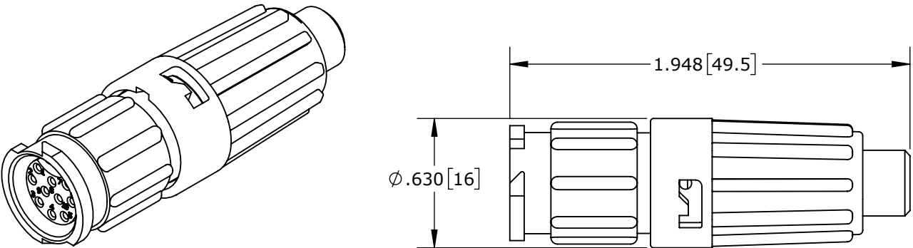
TYPICAL CABLE-TO-CABLE CONNECTOR SHOWN ASSEMBLED
