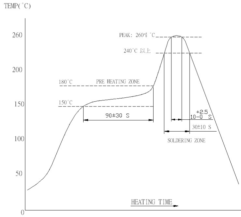
FIGURE IV SOLDERING TEMPERATURE PROFILE
